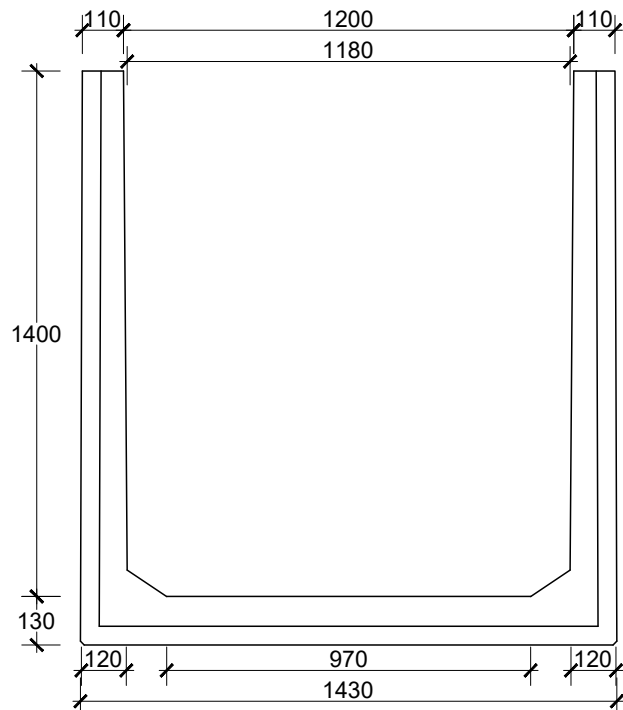
TAMPAK DEPAN U-DITCH 1200 X 1400
