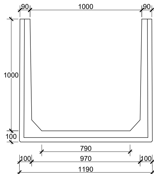
TAMPAK DEPAN U-DITCH 1000 X 1000
