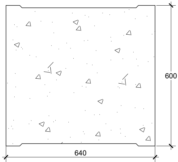
TAMPAK ATAS COVER U-DITCH 500 SKALA 1 : 10
