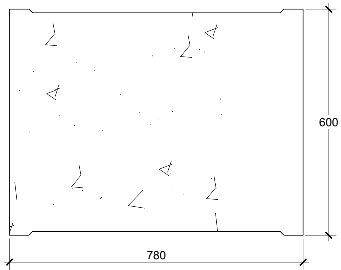
TAMPAK ATAS COVER U-DITCH 400 tb. 40 CM SKALA 1 : 10
