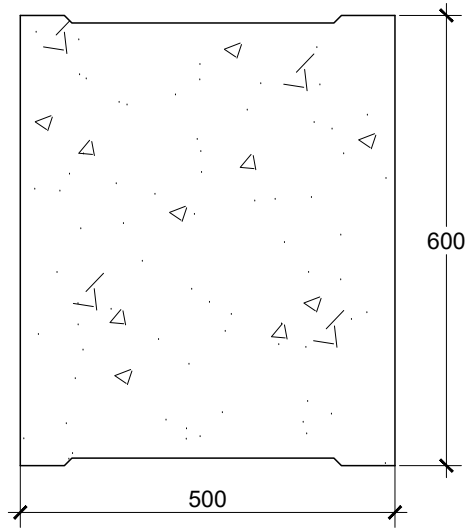
TAMPAK ATAS COVER U-DITCH 400 SKALA 1 : 10
