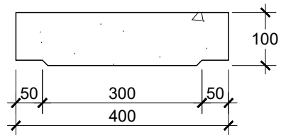
TAMPAK DEPAN COVER U-DITCH 300 SKALA 1 : 10
