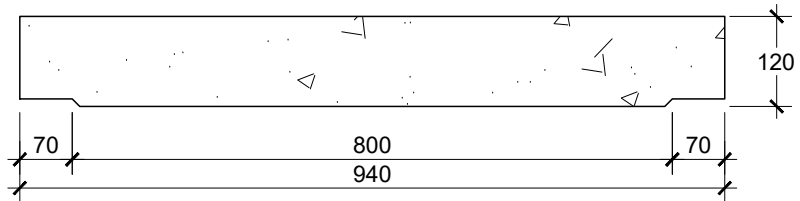
TAMPAK DEPAN COVER U-DITCH 800 SKALA 1 : 10
