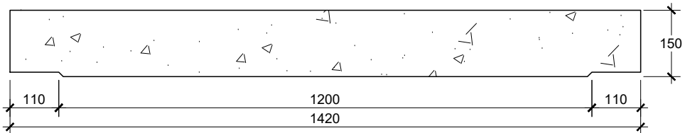
TAMPAK DEPAN COVER U-DITCH 1200 SKALA 1 : 10
