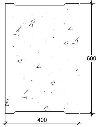
TAMPAK ATAS COVER U-DITCH 300 SKALA 1 : 10
