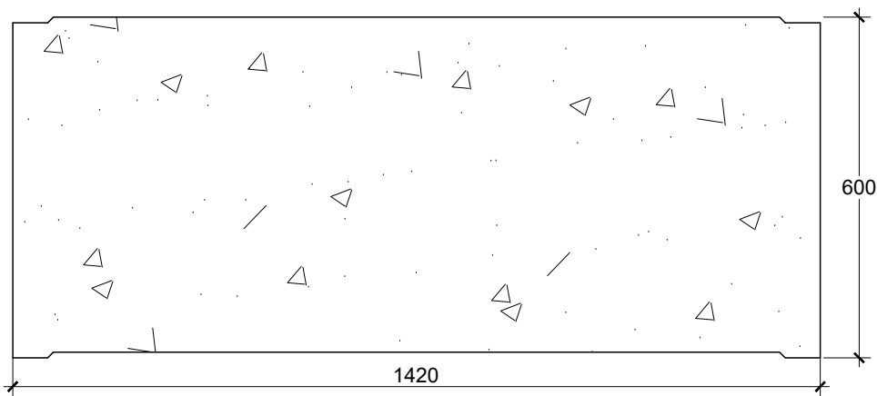
TAMPAK ATAS COVER U-DITCH 1200 SKALA 1 : 10
