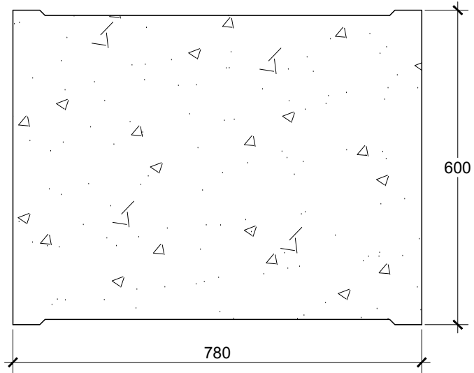
TAMPAK ATAS COVER U-DITCH 400 tb. 30 CM SKALA 1 : 10
