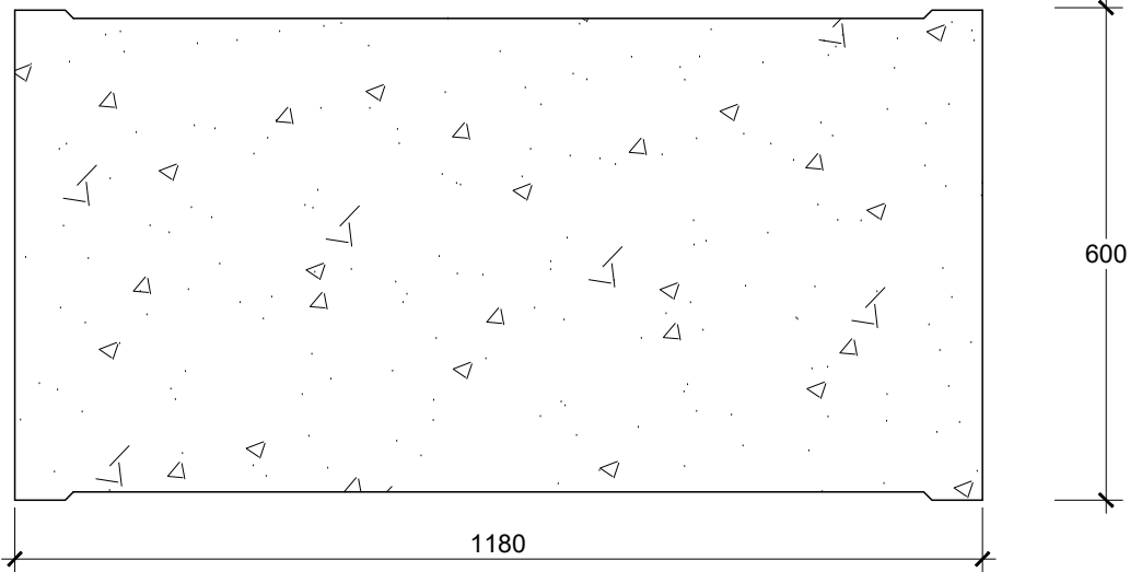
TAMPAK ATAS COVER U-DITCH 1000 SKALA 1 : 10
