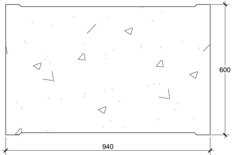
TAMPAK ATAS COVER U-DITCH 800 SKALA 1 : 10
