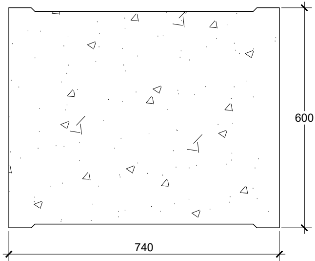
TAMPAK ATAS COVER U-DITCH 600 SKALA 1 : 10
