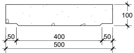
TAMPAK DEPAN COVER U-DITCH 400 SKALA 1 : 10
