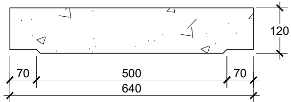
TAMPAK DEPAN COVER U-DITCH 500 SKALA 1 : 10
