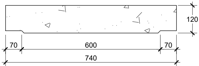
TAMPAK DEPAN COVER U-DITCH 600 SKALA 1 : 10
