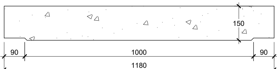
TAMPAK DEPAN COVER U-DITCH 1000 SKALA 1 : 10
