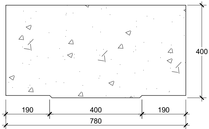
TAMPAK DEPAN COVER U-DITCH 400 tb. 40 CM SKALA 1 : 10
