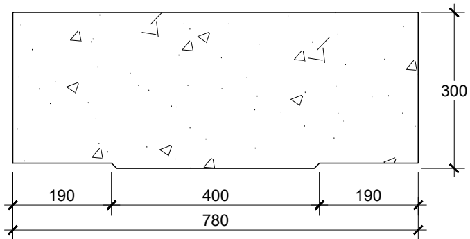
TAMPAK DEPAN COVER U-DITCH 400 tb. 30 CM SKALA 1 : 10
