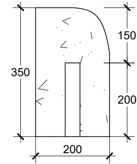
TAMPAK SAMPING KANSTEIN TYPE B SKALA 1 : 10
