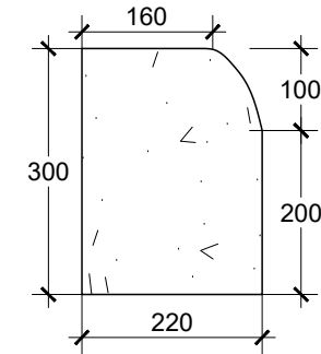
TAMPAK SAMPING KANSTEIN TYPE DKI SKALA 1 : 10
